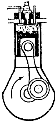
Expansion Stroke (c)
